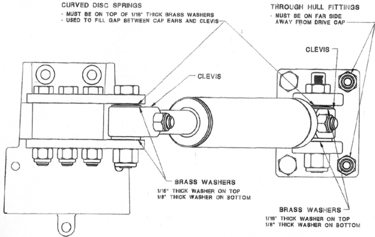
DRIVE CAP / TRANSOM BRACKET STEERING CYLINDER INSTALLATION DRAWING
